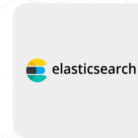
ElasticSearch
