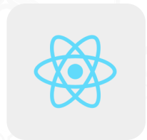
React Native
