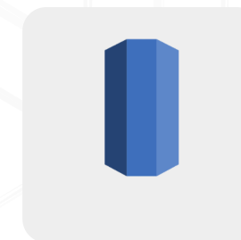
Amazon SimpleDB
